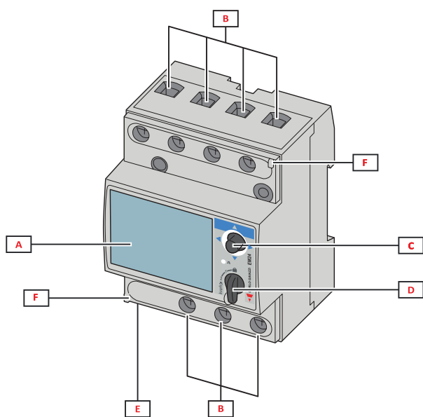
Fig. 1 Direct connection
