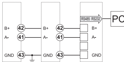
Fig. 29 RS485 port
