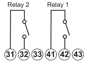
Fig. 27 Relay outputs
